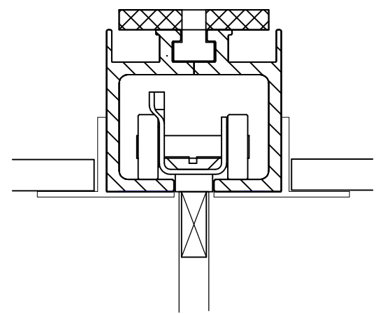
CONCEALED TRACK
